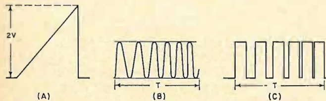
Fig. 6. This shows a greater magnitude of modulating signal. (A) Triangular wave now has peak amplitude of 2V volts. (B) The FM waveform. (C) Twice as many pulses are now counted than for the case where amplitude of the triangular wave was V volts. (In Figs. 5C and 6C, the output pulses are actually negative-going. They are shown inverted to make comparison simpler.)
