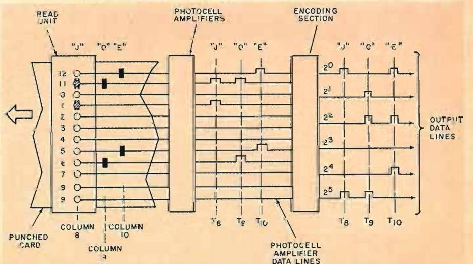
Fig. 5. Data-encoding system that is employed in a photocell reader.
