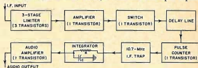
Fig. 2. Block diagram of the new Fisher limiter-detector circuit.
