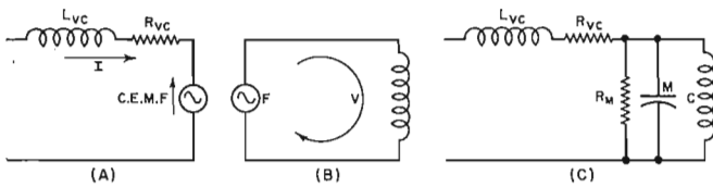
Fig. 2. Electrical and mechanical equivalent circuits of speaker.
