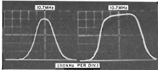
Fig. 3. Over-all i.f. bandpass of another receiver with normal input signal (left) and with much higher amplitude input (right).
