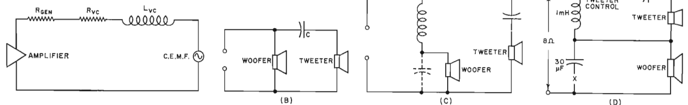
Fig. 4. (A) Equivalent circuit of speaker connected to amplifier. (B), (C), and (D) Two-way speaker systems and networks.
